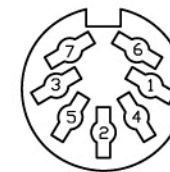
7 pin
