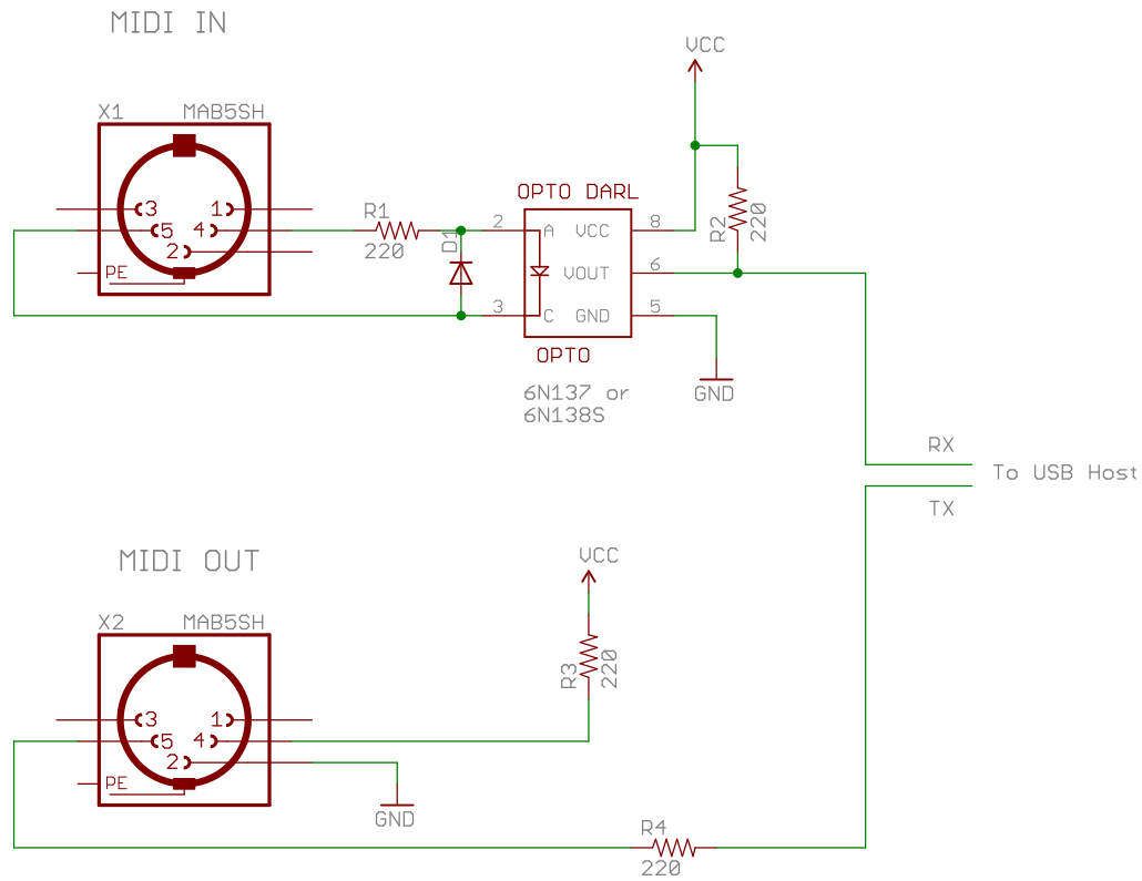
Serial MIDI connections to USB Host board/chips
